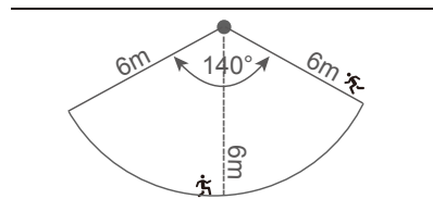
Sensing Distance
