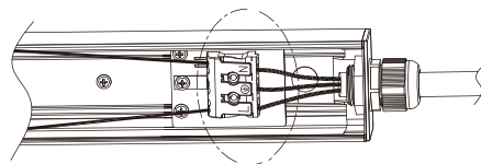
Side wiring
